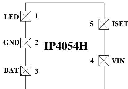
Figure 2 Pin of IP4054H
