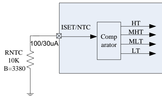
Figure 6 NTC Diagram
