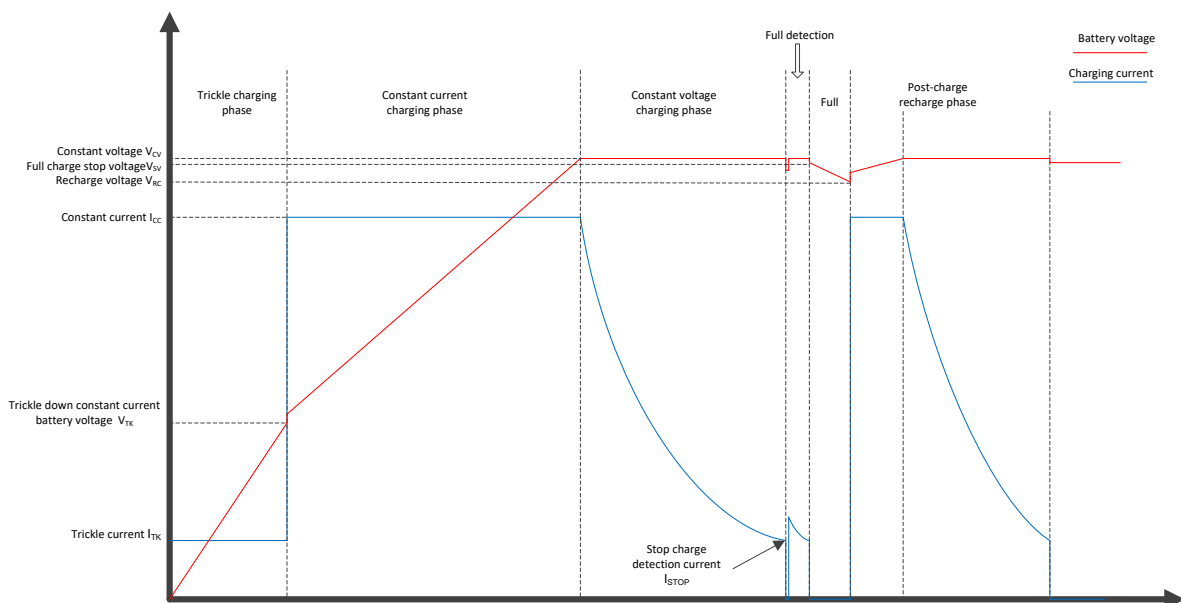
Figure 4 IP4054H Schematic diagram of the charging process
