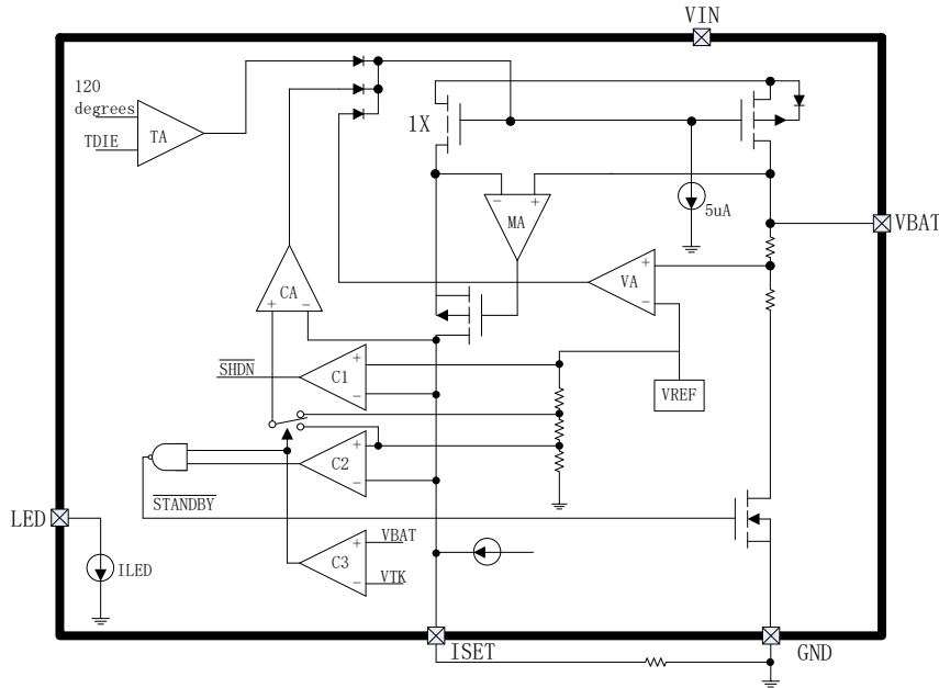
Figure 3 IP4054H Functional Block Diagram
