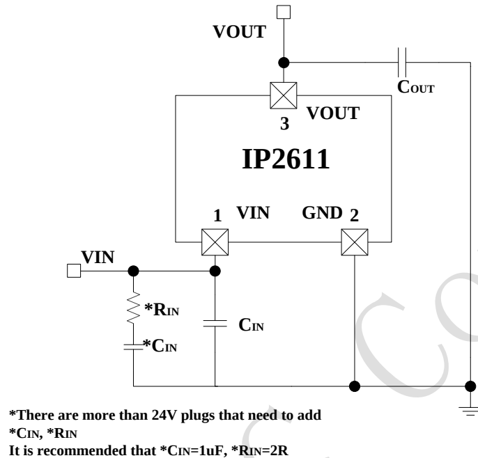
Figure10 Typical application schematic
