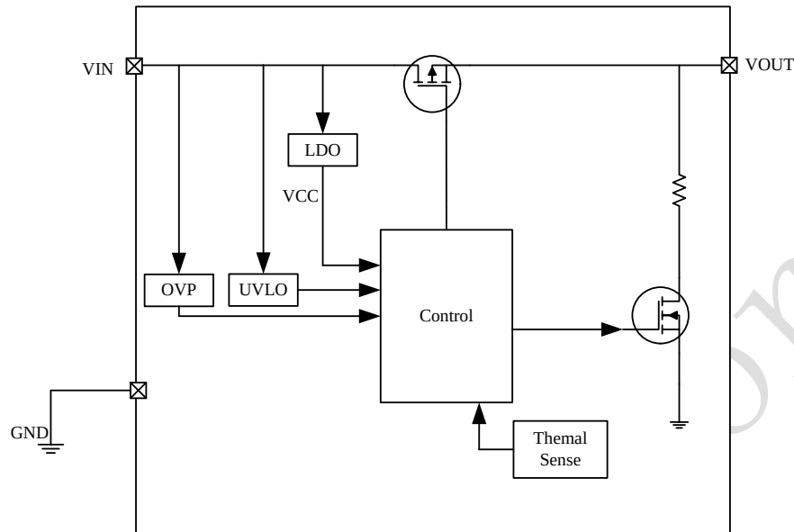
Figure3 Internal block diagram of IP2611
