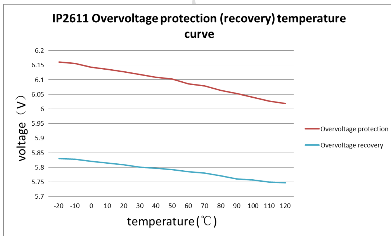
Figure9 voltage protection (recovery) temperature curve
