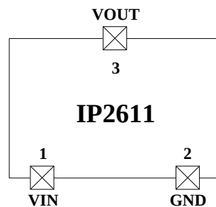
Figure2 Pin of IP2611
