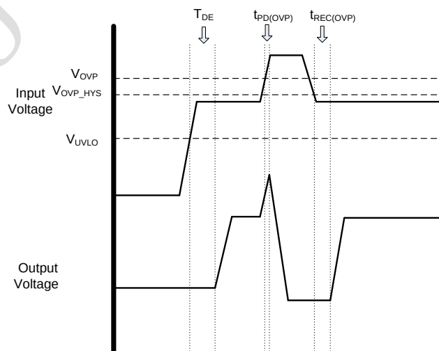
Figure4 timing diagram
